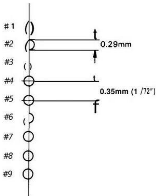
Figure 1-2. Pin Configuration
